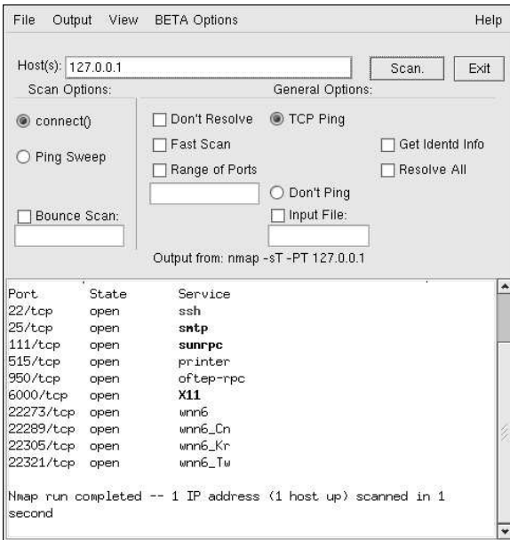
Figure 8-1. Scanning with Nmap
