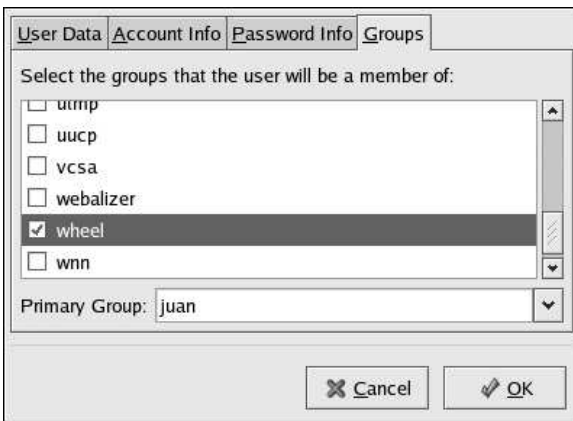
Figure 4-2. Groups Pane
